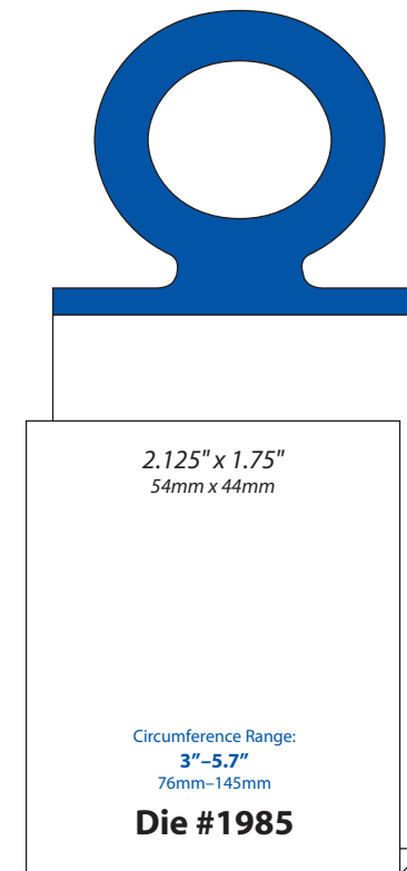
FOLDED FRONT VIEW
