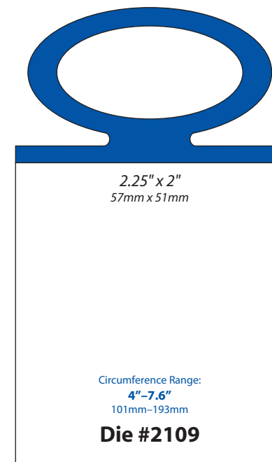
Single/Bifold Same as standard die 1946
