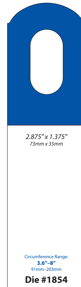
Single Same as spooled die 1989
